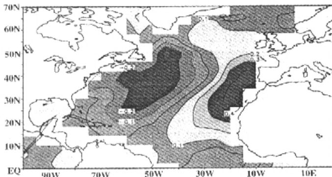
Fig. 3 Correlation between the observed NAO and SST anomaly [53] .
